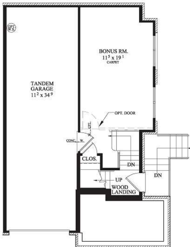
Basement 714 SQ. FT.
