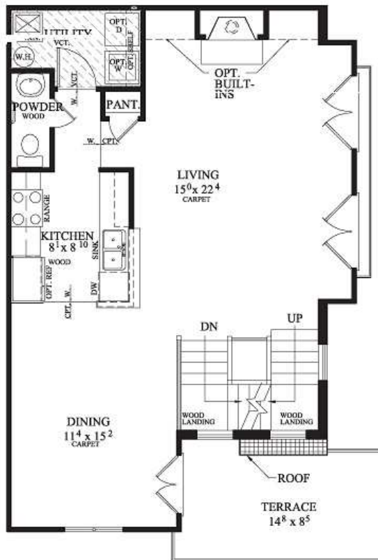
First Floor 720 SQ. FT.
