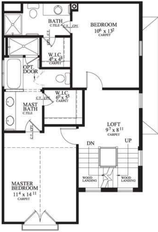
Second Floor 668 SQ. FT.
