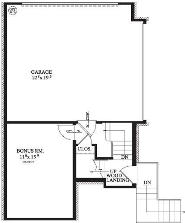
Basement 715 SQ. FT.
