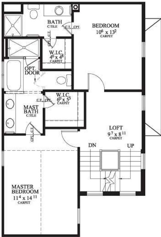
Second Floor 683 SQ. FT.
