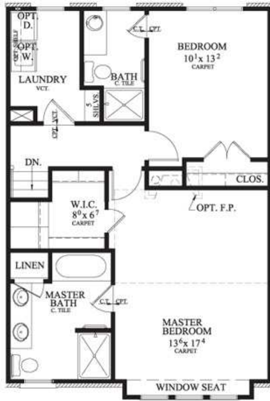
Second Floor 689 SQ. FT.
