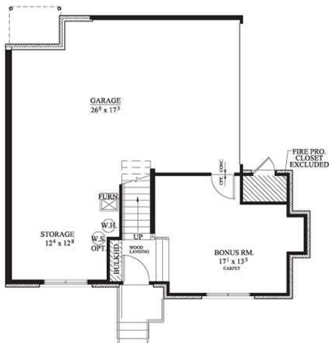
Basement 844 SQ. FT.
